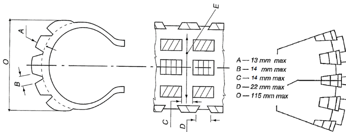
Figure 3 : Tyre dimensions
